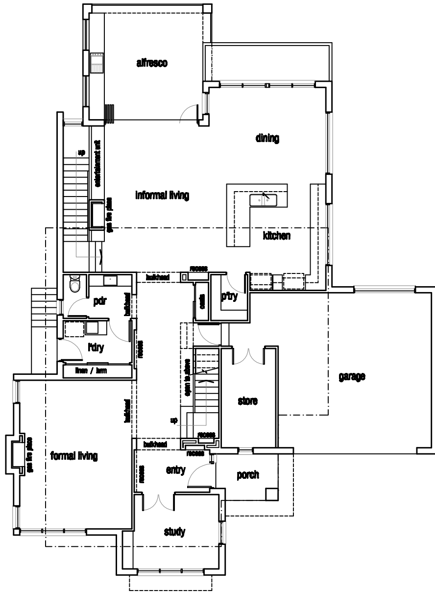
upper ground floor plan 1:100
